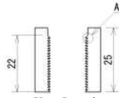
Vise Jaws for GT-30-E
