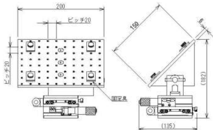
XY table for QFP lead test
