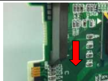
A component is pressed with GT-20 to test shear strength.
