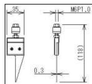
QFP lead hook
