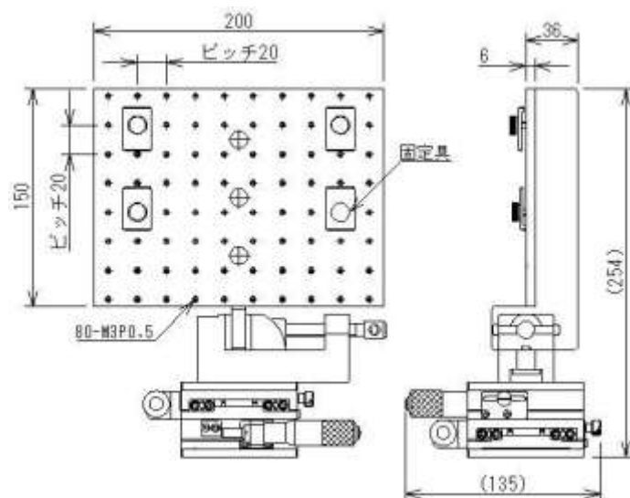
XY table for soldering shearing test
