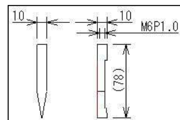
Soldering shearing jig
