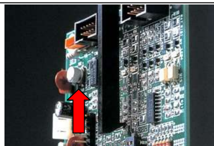
A component is pulled up with GT-10 to test its peel strength.
